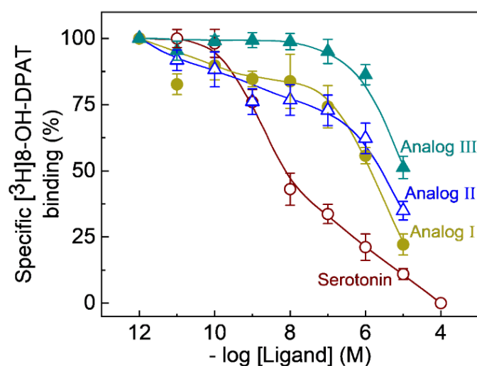
Figure 2. Competition binding of fluorescent NBD-labeled serotonin ligands to the human serotonin 1A receptor stably expressed in CHO-K1 cells. Radioligand binding assays were carried out with [ 3 H]8-OH-DPAT in the presence of a range of concentrations (from 10^{-12} to 10^{-4} M) for serotonin (○) and NBD-labeled analogs I (●), II (△) and III (▲). Values of specific binding measured in the presence of fluorescent analogs are expressed as a percentage of total binding obtained at the lowest concentration of the competing ligand. The curves represent nonlinear regression fits to the experimental as described in the Supplementary Material. Data shown are means \pm SE from five independent experiments. Nonspecific binding was determined in the presence of 10^{-4} M unlabeled serotonin in each case. K_i values were determined according to Cheng and Prusoff [60] and the average values are listed in Table 1. See Materials and Methods for other details.
