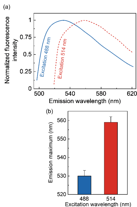
Figure 7. (a) Representative fluorescence emission spectra of NBD-serotonin analog I bound to the serotonin 1A receptor expressed in CHO-K1 cells at different excitation wavelengths. The excitation wavelengths were 488 (—) and 514 (---) nm. All spectra are intensity-normalized at the emission maximum. The concentration of NBD-serotonin analog I was 7 \mu M. A Zeiss LSM 880 inverted spectral imaging confocal microscope with a multichannel spectral detector was used to construct pixel-by-pixel fluorescence emission spectra from the confocal images. (b) Effect of changing excitation wavelength on the wavelength of maximum emission for NBD-serotonin analog I. Data represent means \pm SE of at least 35 different fields from three independent experiments. See Materials and Methods for other details.
