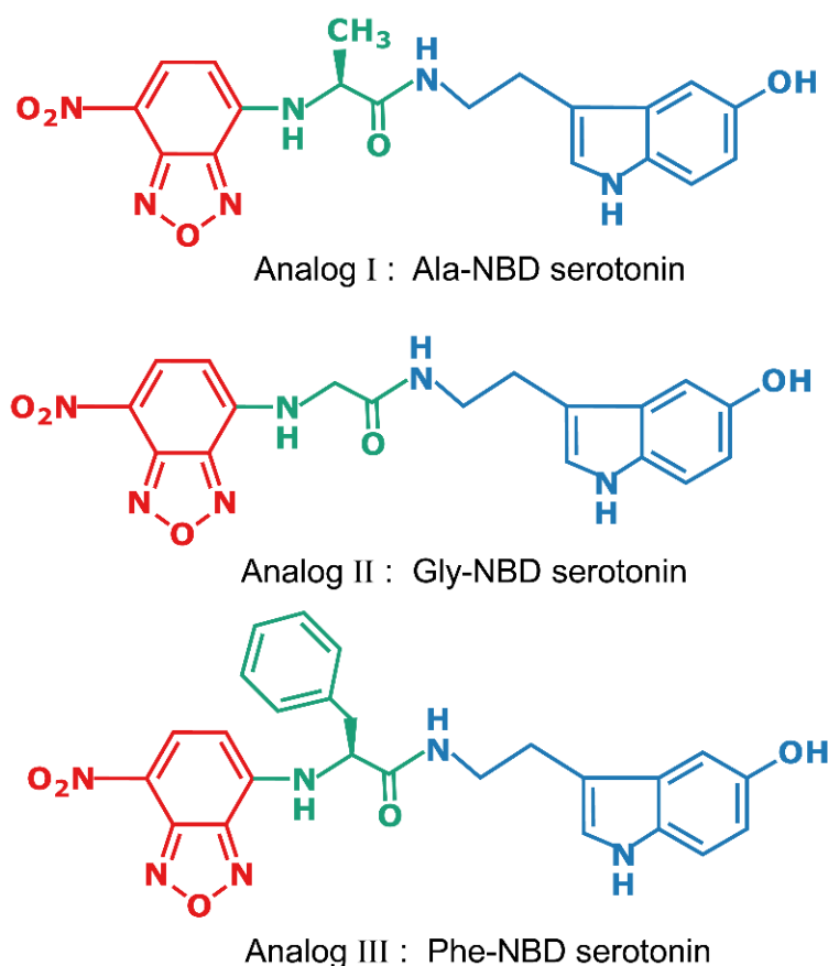
Figure 1. Chemical structures of the fluorescent NBD-labeled analogs of serotonin used in this study. The fluorophore (NBD) is shown in red, serotonin is shown in blue, and the linker amino acid is depicted in green.
