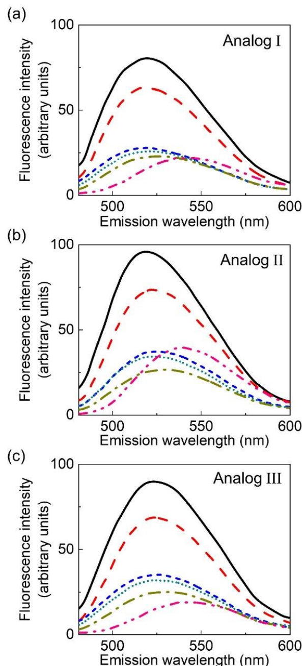
Figure 3. Fluorescence emission spectra of NBD-labeled analogs of serotonin (I–III) in solvents of varying polarity shown in panels (a–c), respectively. The solvents used were tetrahydrofuran (—), acetone (---), isopropanol (·····), ethanol (— · — ·), methanol (— — —), and dimethyl sulfoxide (— · — ·). The concentration of the NBD analogs of serotonin used was 8 \mu M and the excitation wavelength used was 465 nm in all cases. See Materials and Methods for other details.
