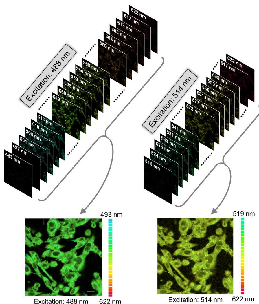
Figure 6. Spectral image stacks consisting of a collection of images showing serotonin 1A receptor labeled using NBD-serotonin analog I, each of which measured at a specific wavelength (highlighted on top left corner of image) for two different excitation wavelengths. Unlike a typical confocal image, which is acquired over a wavelength range of the detector, a spectral image contains a collection of images of the same field captured at different wavelengths. As a result, spectral images provide a complete emission spectrum of the fluorophore at every pixel location. The corresponding overlaid image of the linearly unmixed spectral image stack is shown at the bottom. The individual images in the stack were colored according to the color-map showed beside the overlaid image. Note that the overall red-shifted emission of the NBD-serotonin analog I when excited at the red edge (514 nm) indicates REES. The scale bar represents 10 \mu m. See Materials and Methods for other details.
