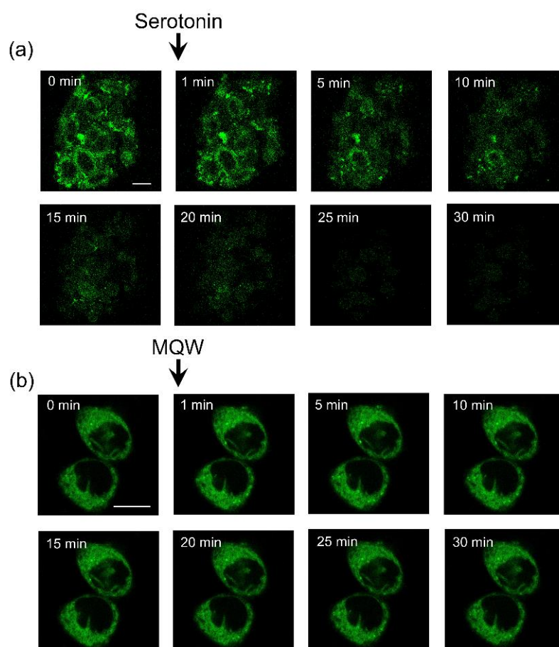
Figure 5. (a) Confocal microscopic images of the human serotonin 1A receptor stably expressed in CHO-K1 cells labeled with the NBD-labeled analog of serotonin (I) and chased with unlabeled serotonin. Images represent mid-plane confocal sections of the same group of cells before and after addition of serotonin. Cells were initially labeled with 7 \mu M of analog I in HEPES-HANKS buffer, pH 7.2 and subsequently serotonin (final concentration 7 mM) was added at 1 min time point (indicated by an arrow) from a concentrated aqueous stock solution. (b) Control experiment showing confocal microscopic images of the serotonin 1A receptor stably expressed in CHO-K1 cells labeled with the NBD-labeled analog of serotonin (I) and chased with same volume of Milli-Q water (MQW) as in panel (a). Images represent mid-plane confocal sections of the same group of cells before and after addition of MQW. Scale bars represent 10 \mu m. See Materials and Methods for other details.
