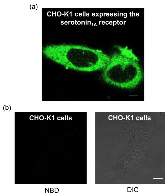
Figure 4. (a) Confocal microscopic images obtained by specific labeling of the serotonin 1A receptor stably expressed in CHO-K1 cells with the NBD-labeled analog of serotonin (I). Cells were grown on Lab-Tek chambers and labeled with 7 \mu M of analog I in HEPES-HANKS buffer, pH 7.2. NBD was excited using a 488 nm argon laser and emission was collected between 505–600 nm. Panel (b) shows background fluorescence of untransfected CHO-K1 cells (lacking the serotonin 1A receptor) labeled with 7 \mu M of analog I under the same conditions as in panel (a). The right panel shows DIC image. Scale bars represent 10 \mu m. See Materials and Methods for other details.
